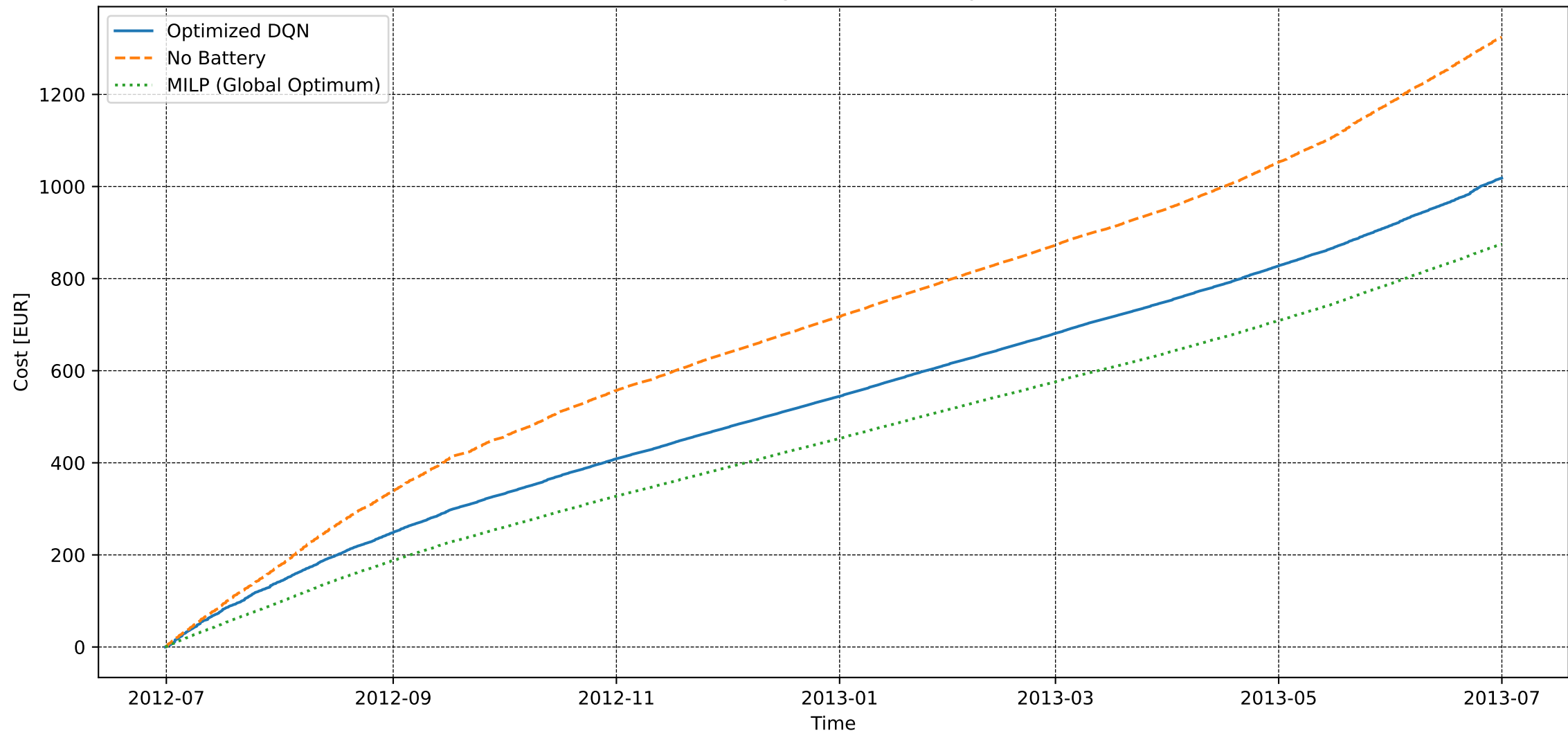
User 223 - Extended Convergence - Electricity Cost [DQN vs MILP]
